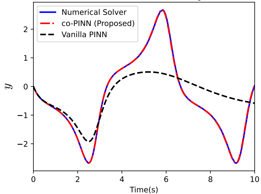
Oscillator Velocity
