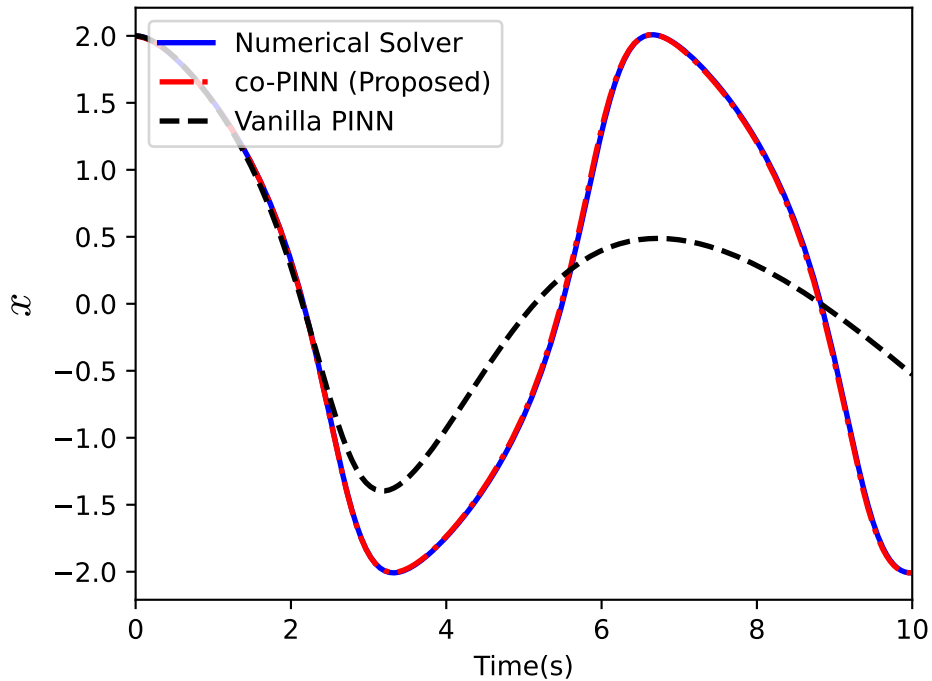
Oscillator Position
