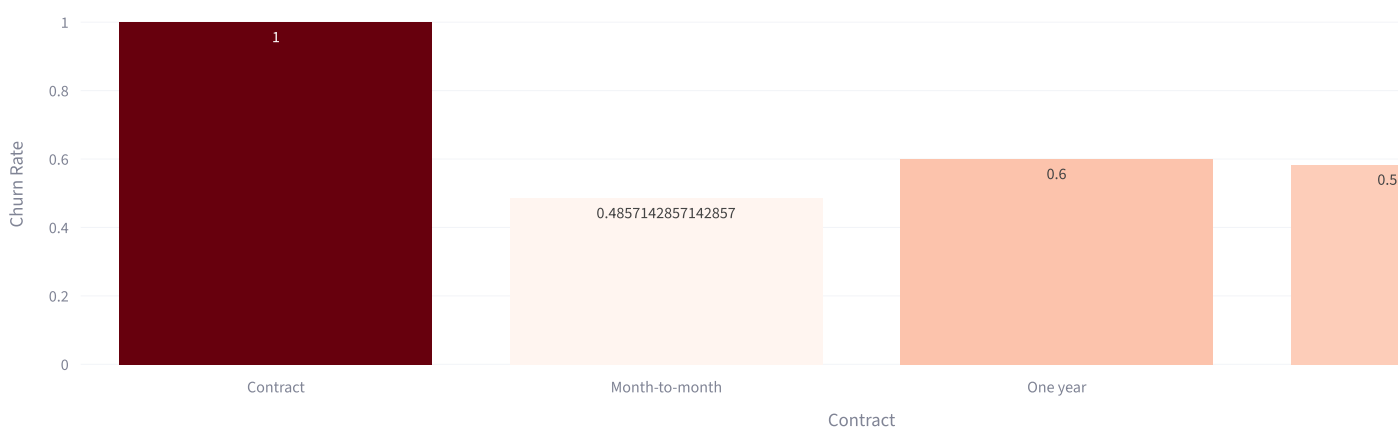
Average Churn Rate by Contract Type
