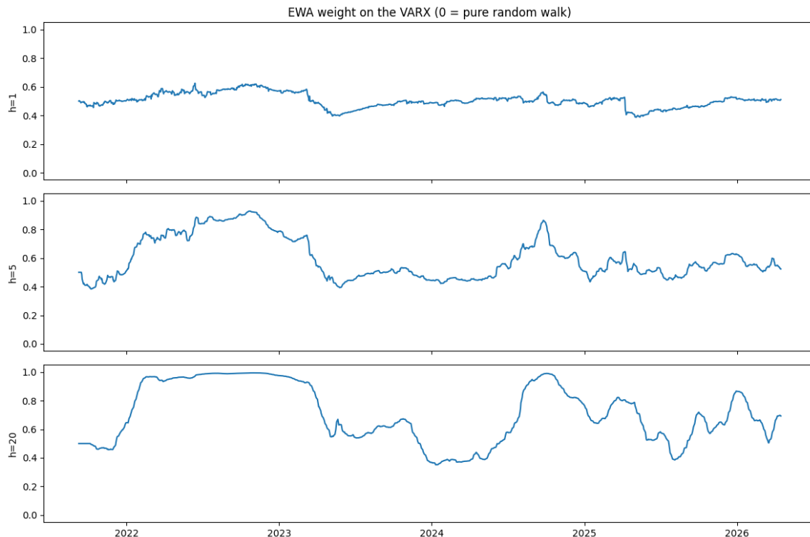
Figure 3: EWA combination weight on the VARX at each evaluation date, by horizon. A value of zero corresponds to the pure random walk. The weight rises toward one through the 2022 tightening cycle and retreats in directionless periods.
