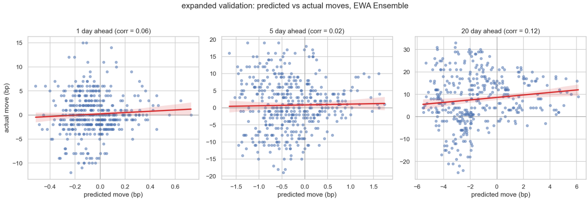
Figure 5: Validation on post-development data: predicted versus realized yield moves for the EWA ensemble by horizon, with fitted relationships. Correlations are 0.06, 0.02, and 0.12, reflecting the sharp July 2026 reversal that the adaptive system did not anticipate.
