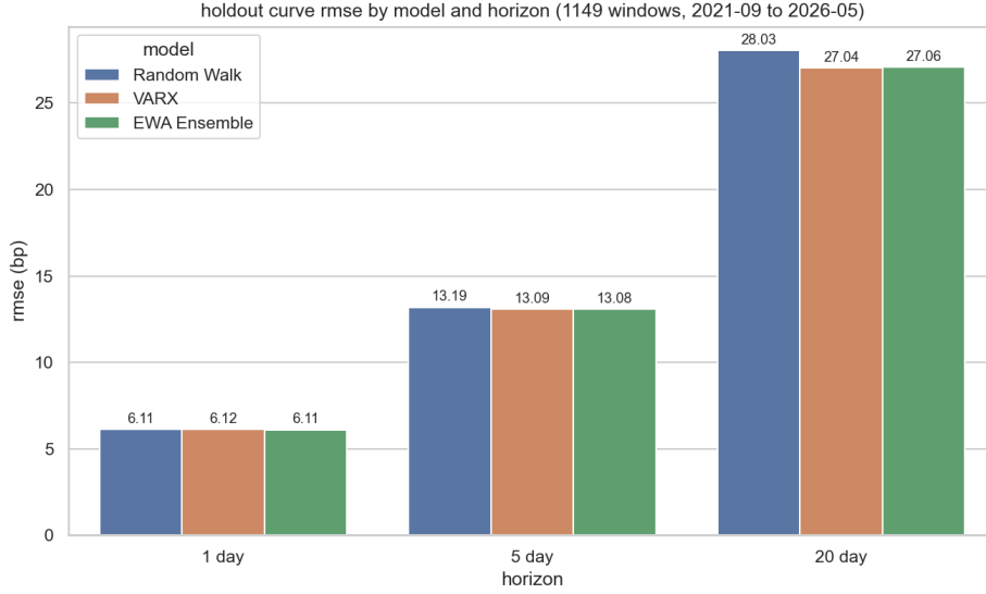
Figure 1: Curve RMSE by model and horizon over the 1,149-window holdout. Differences are small in absolute terms and grow with horizon.
