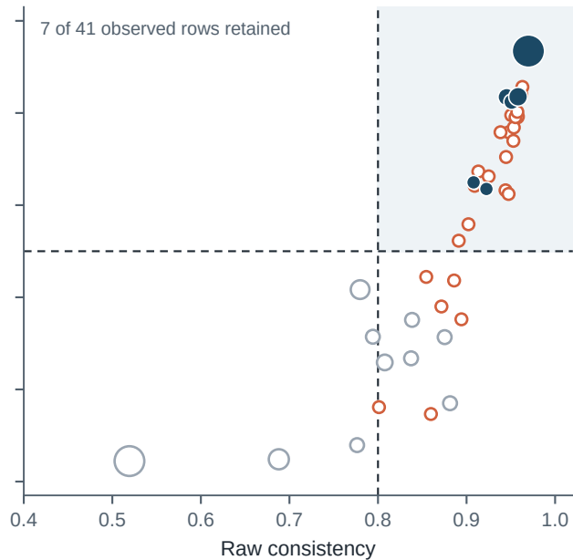
Percentile calibration
