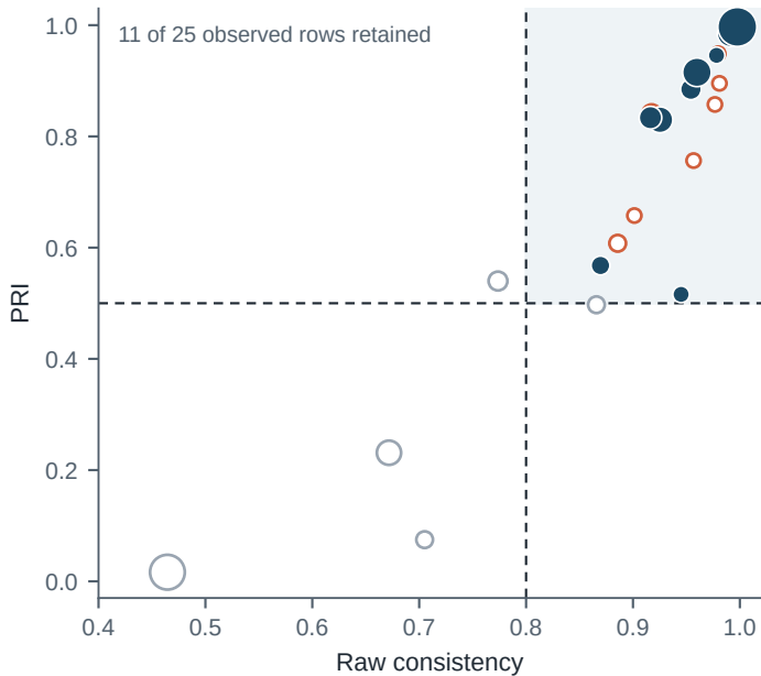
Rubric calibration
