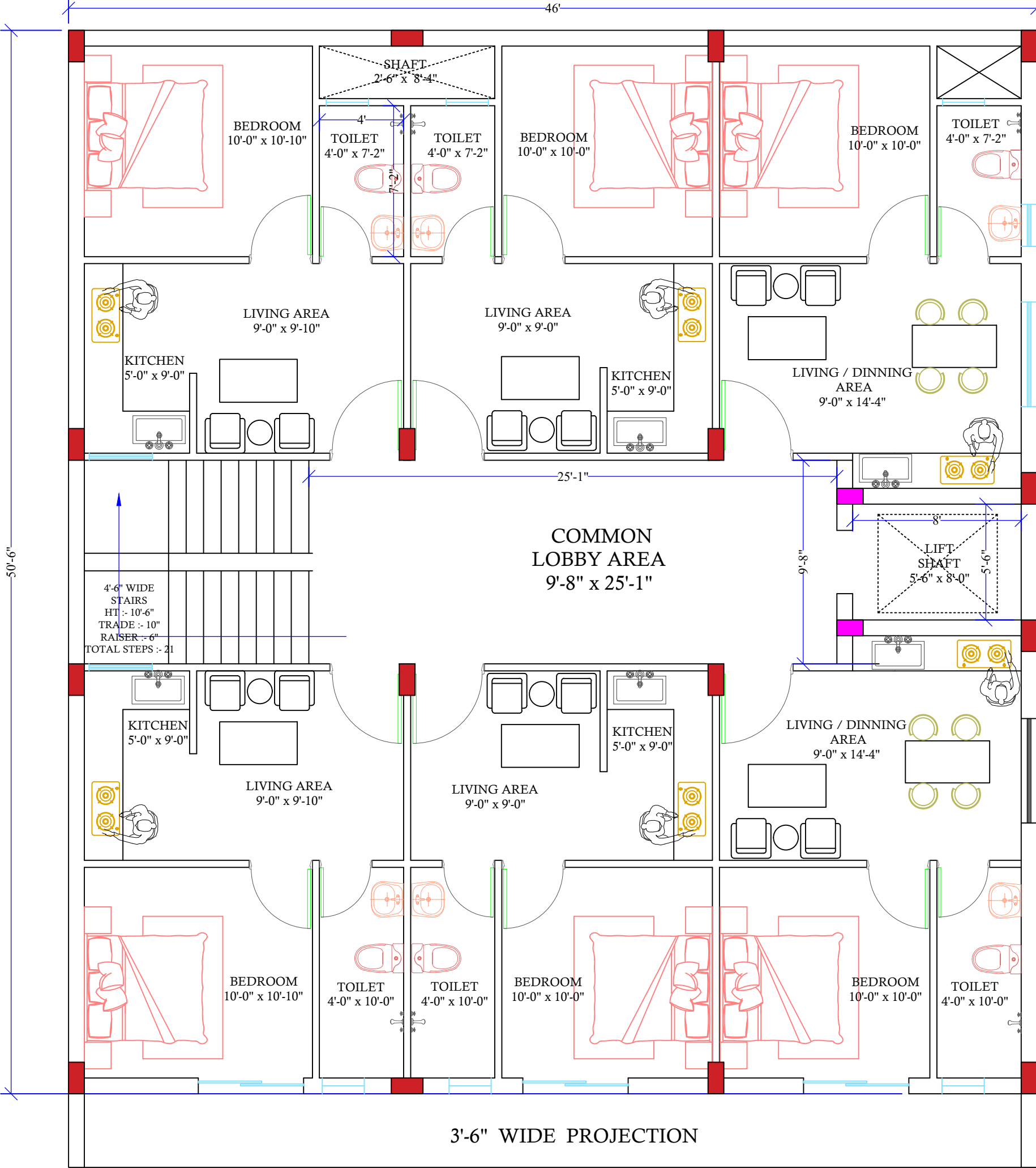
TYPICAL FLOOR
