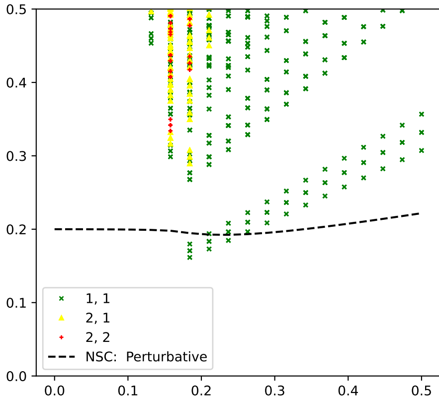
Results 2Exc-1Imp continuum: \mu/U = 0.41 , U/B/U = 0.20 , Total Sites = 196
