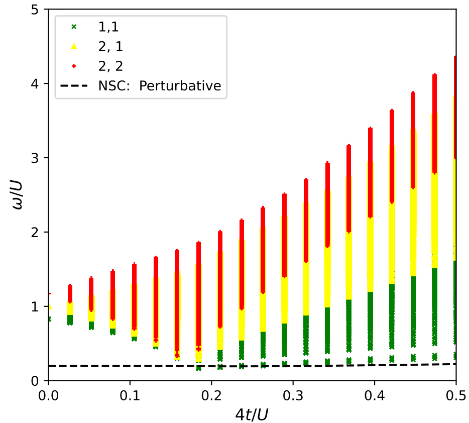
Results 2Exc-1Imp continuum: \mu/U = 0.41 , U/B/U = 0.20 , Total Sites = 196
