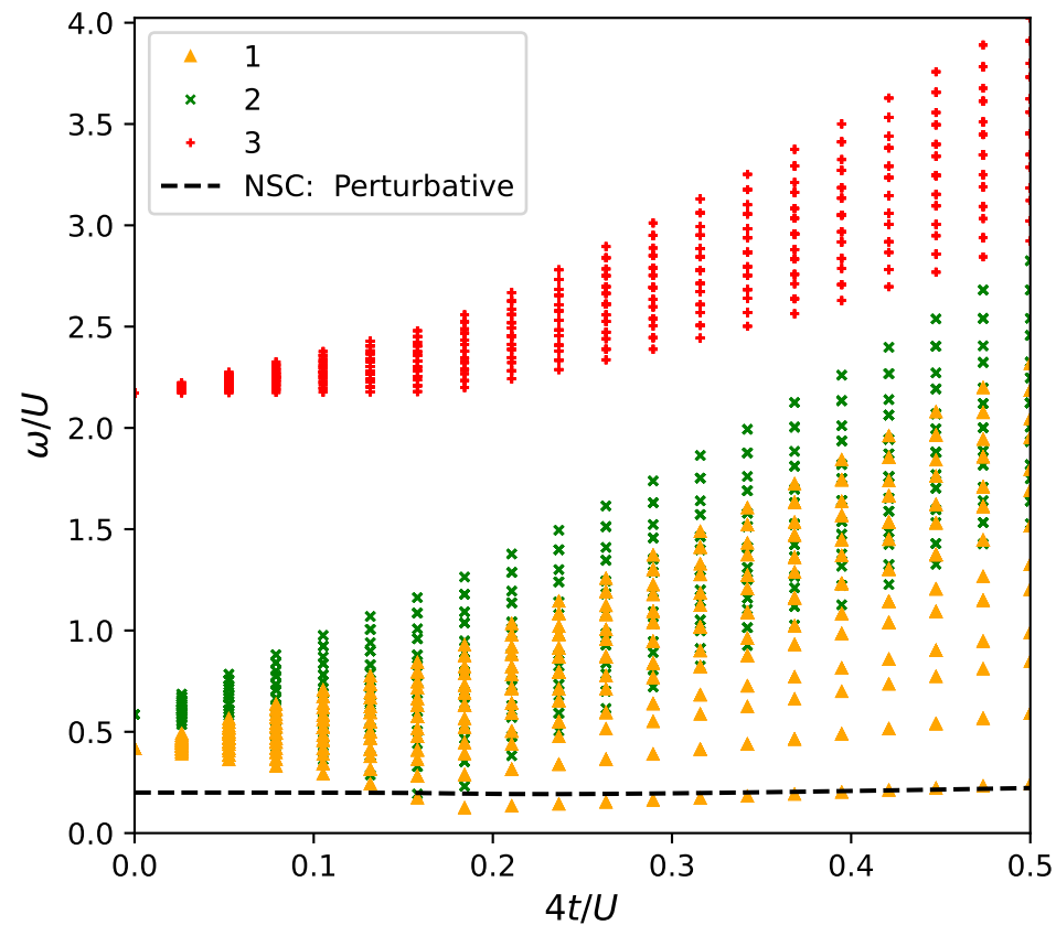
Results 1Exc-1Imp continuum: \mu/U = 0.41 , U\Gamma/U = 0.20 , Total Sites = 100
