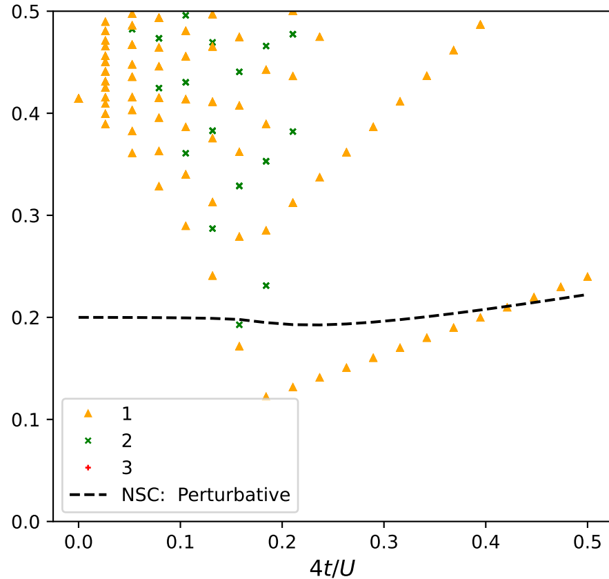
Results 1Exc-1Imp continuum: \mu/U = 0.41 , U\Gamma/U = 0.20 , Total Sites = 100
