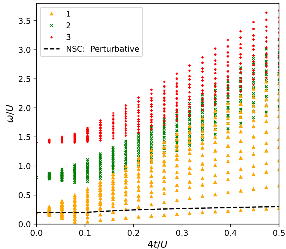
Results 1Exc-1Imp continuum: \mu/U = 0.80 , U_{IB}/U = 0.20 , Total Sites = 100
