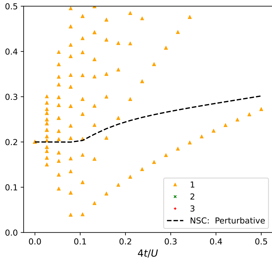
Results 1Exc-1Imp continuum: \mu/U = 0.80 , U_{IB}/U = 0.20 , Total Sites = 100
