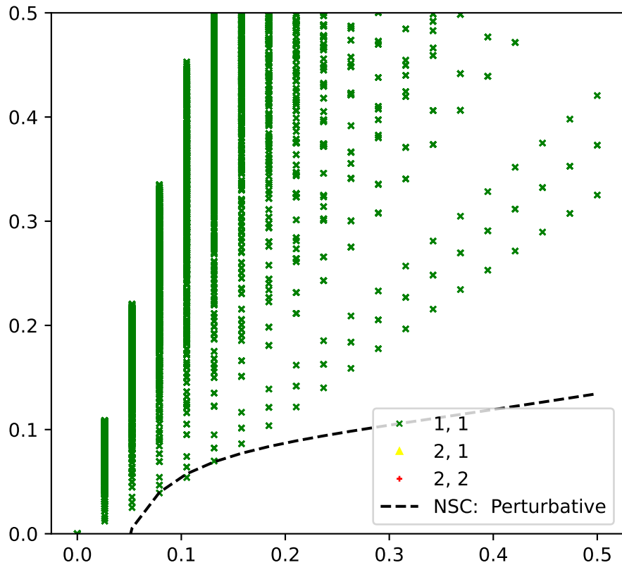
Results 2Exc-1Imp continuum: \mu/U = 0.00 , U_{IB}/U = 0.20 , Total Sites = 100
