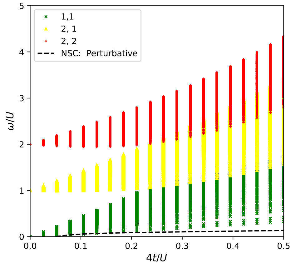
Results 2Exc-1Imp continuum: \mu/U = 0.00 , U_{IB}/U = 0.20 , Total Sites = 100
