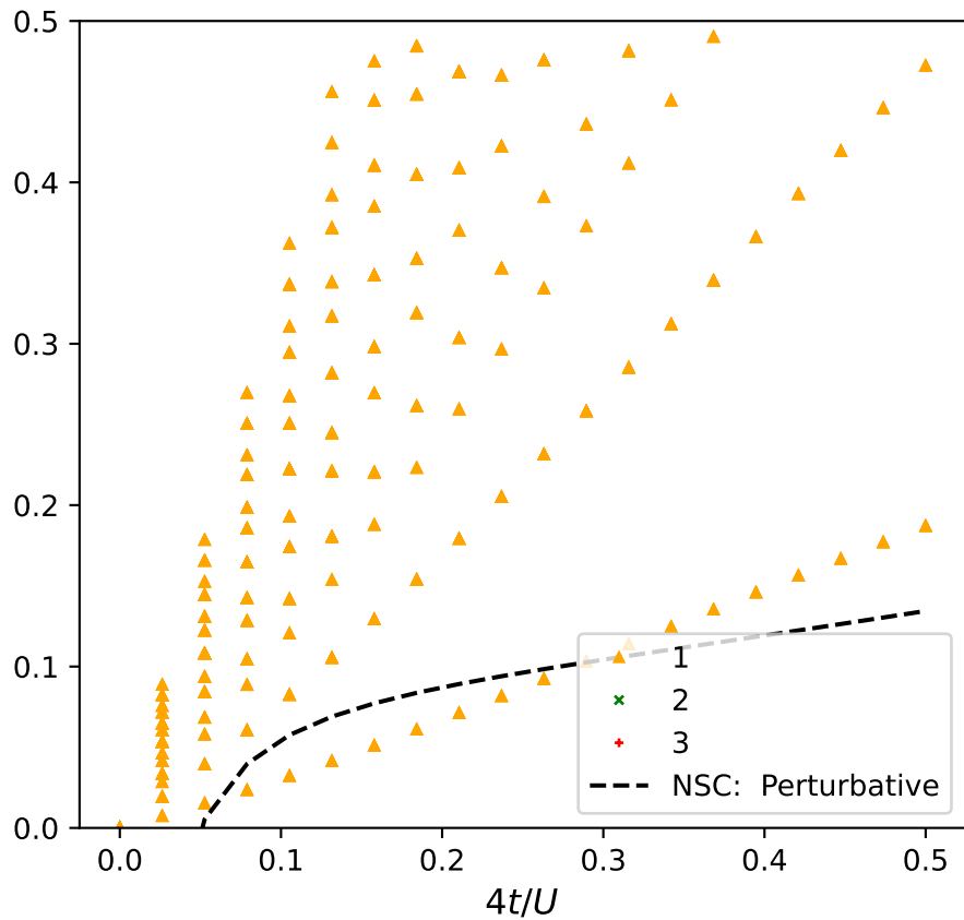
Results 1Exc-1Imp continuum: \mu/U = 0.00 , U_{IB}/U = 0.20 , Total Sites = 100
