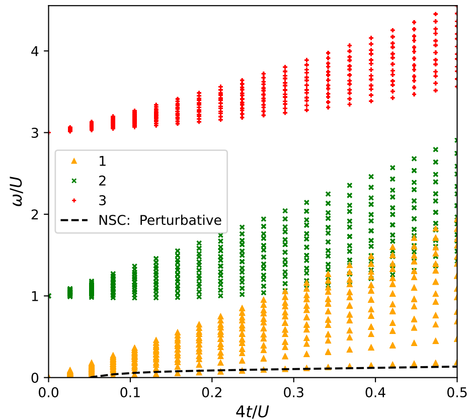
Results 1Exc-1Imp continuum: \mu/U = 0.00 , U_{IB}/U = 0.20 , Total Sites = 100
