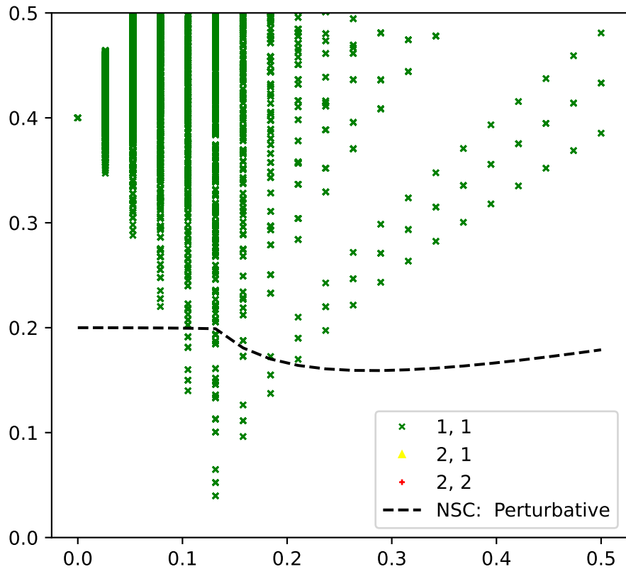
Results 2Exc-1Imp continuum: \mu/U = 0.20 , U_{IB}/U = 0.20 , Total Sites = 100
