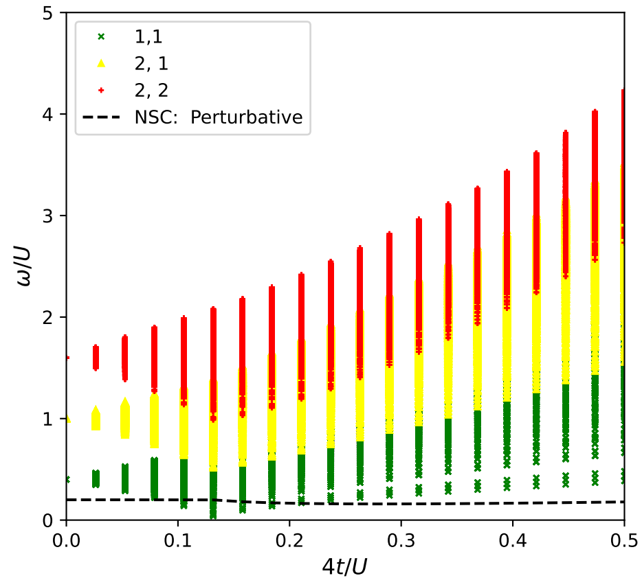
Results 2Exc-1Imp continuum: \mu/U = 0.20 , U_{IB}/U = 0.20 , Total Sites = 100
