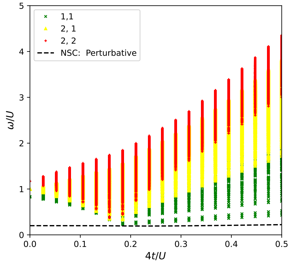
Results 2Exc-1Imp continuum: \mu/U = 0.41 , U_B/U = 0.20 , Total Sites = 100
