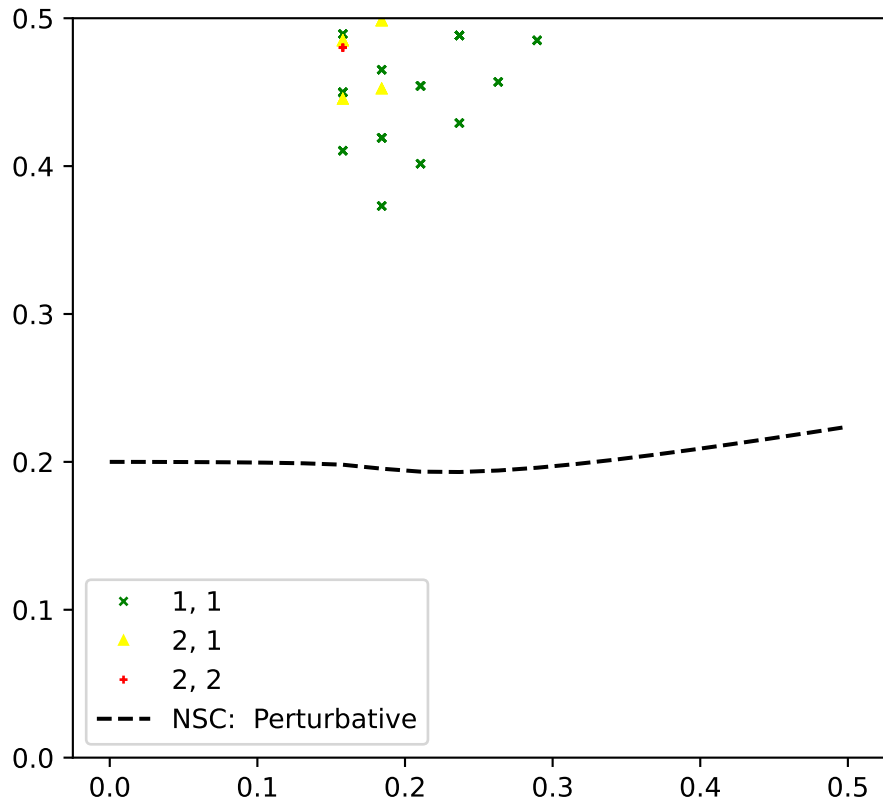
Results 2Exc-1Imp continuum: \mu/U = 0.41 , U/B/U = 0.20 , Total Sites = 36
