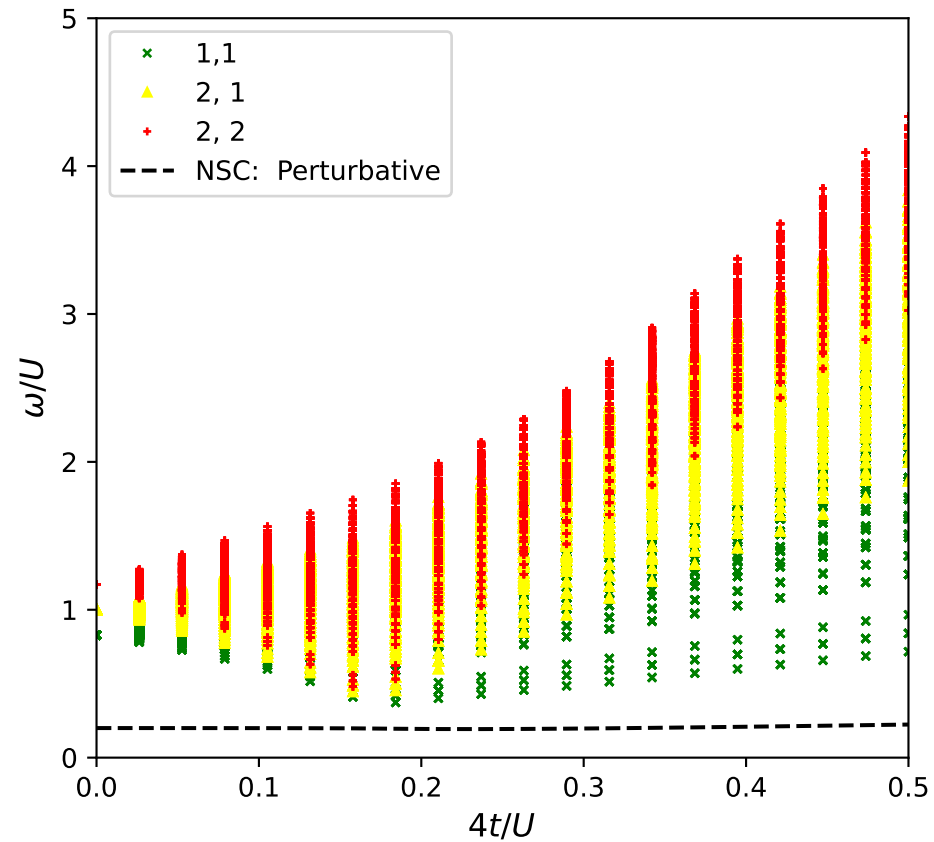
Results 2Exc-1Imp continuum: \mu/U = 0.41 , U/B/U = 0.20 , Total Sites = 36
