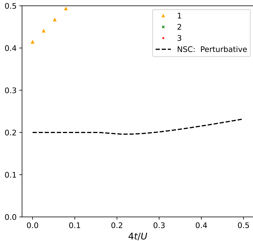
Results 1Exc-1Imp continuum: \mu/U = 0.41 , U/B/U = 0.20 , Total Sites = 4
