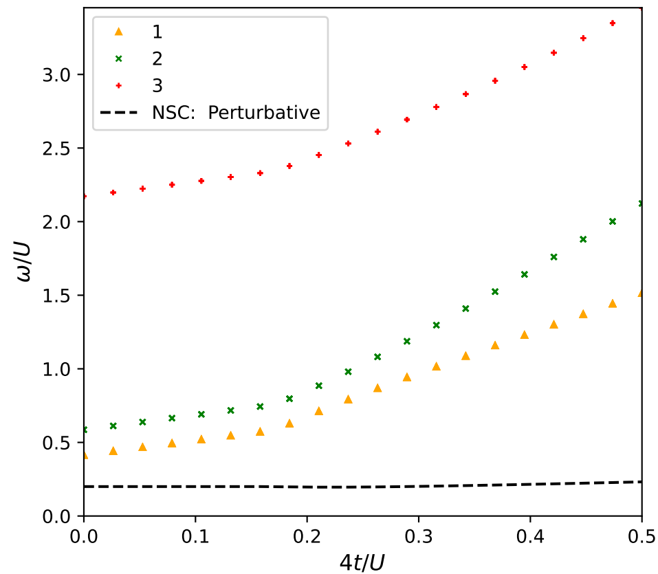
Results 1Exc-1Imp continuum: \mu/U = 0.41 , U/B/U = 0.20 , Total Sites = 4
