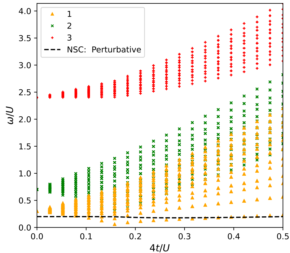
Results 1Exc-1Imp continuum: \mu/U = 0.30 , U_B/U = 0.20 , Total Sites = 100
