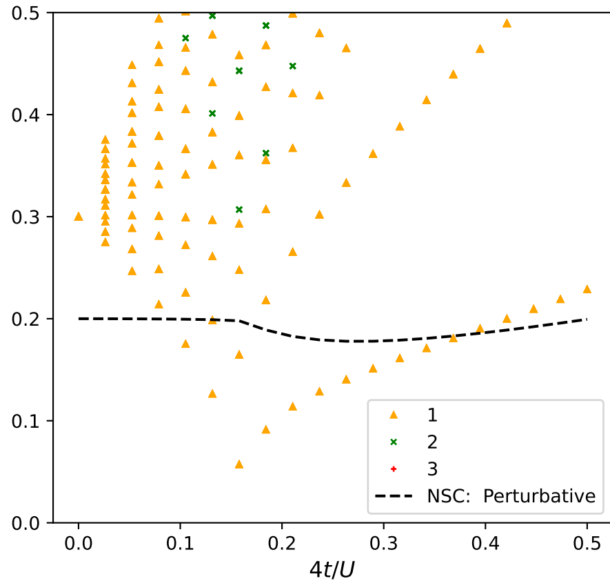
Results 1Exc-1Imp continuum: \mu/U = 0.30 , U_B/U = 0.20 , Total Sites = 100
