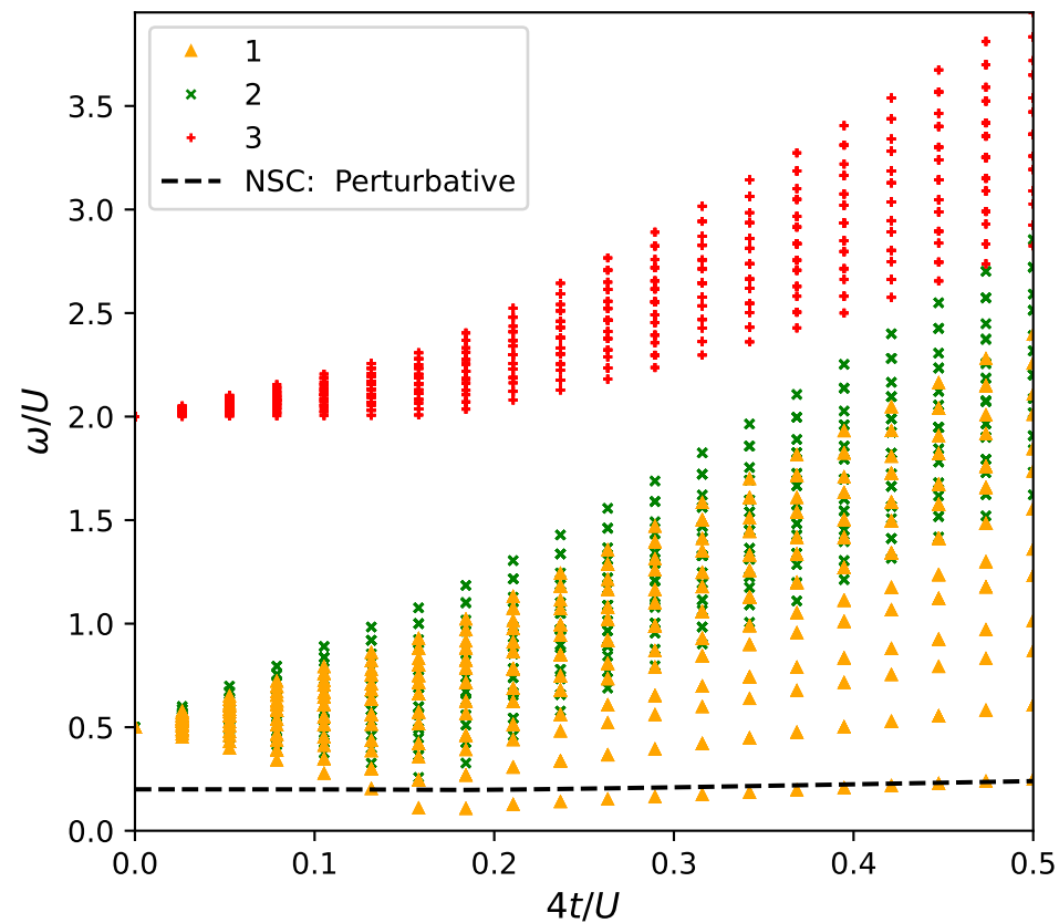
Results 1Exc-1Imp continuum: \mu/U = 0.50 , U/B/U = 0.20 , Total Sites = 100
