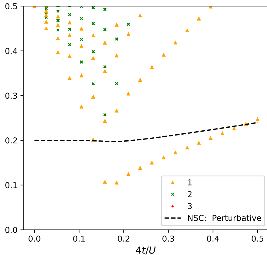
Results 1Exc-1Imp continuum: \mu/U = 0.50 , U/B/U = 0.20 , Total Sites = 100
