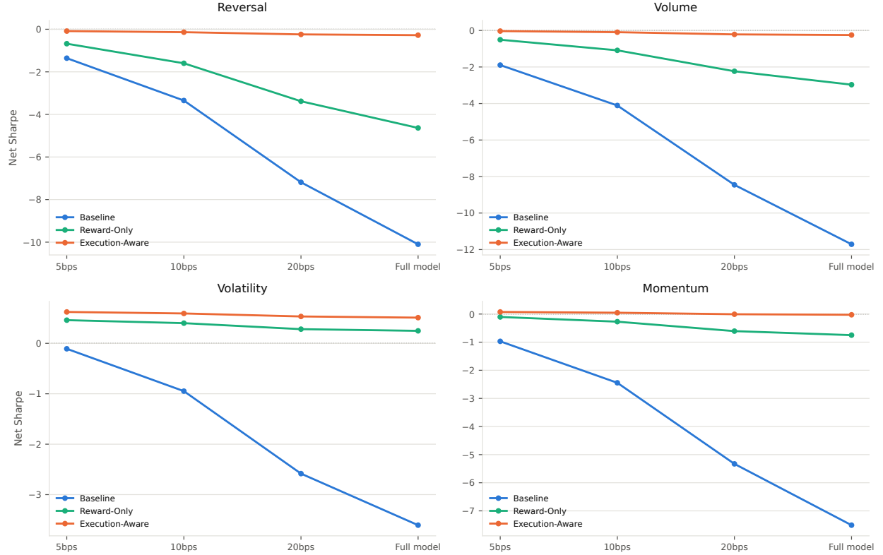
Figure 3: Net Sharpe ratio under alternative cost assumptions. Flat one-way costs of 5, 10 and 20 basis points and the full spread-and-impact model, averaged across the three LLM sampling seeds.
