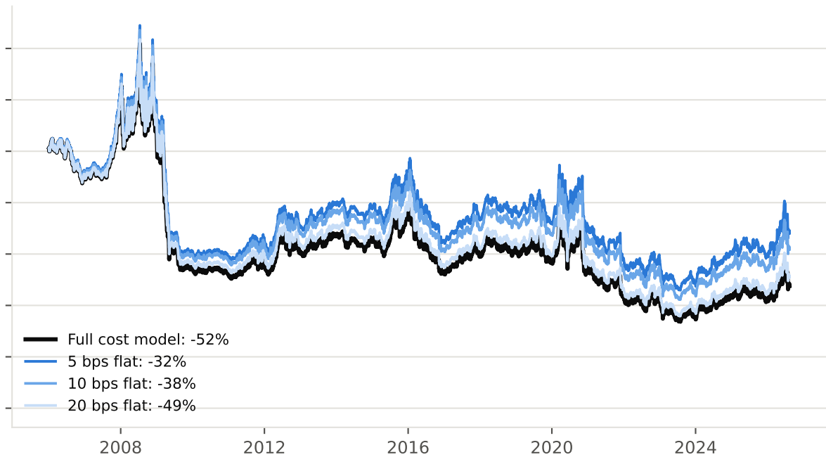
Execution-Aware
