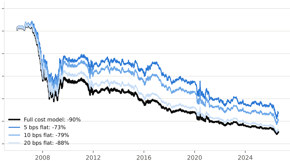
Execution-Aware
