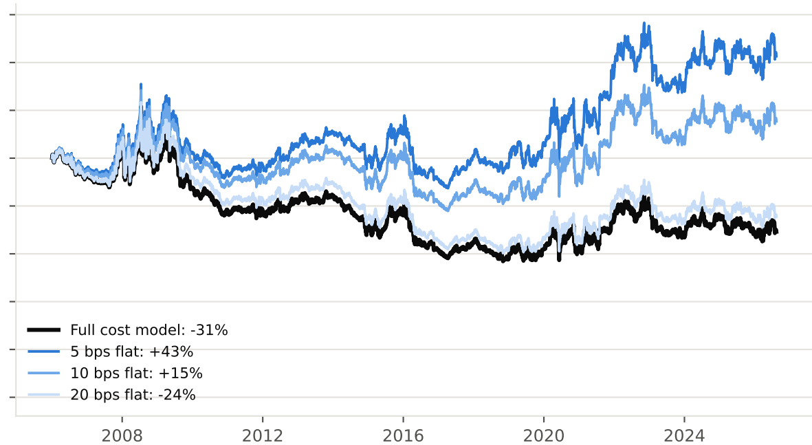
Execution-Aware
