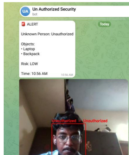
Telegram Alert
