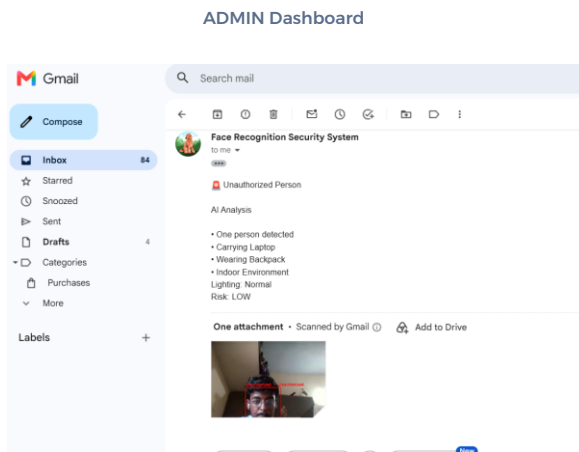
Email Alert
