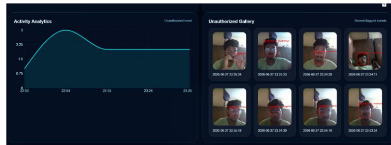
Unauthorized Gallery
