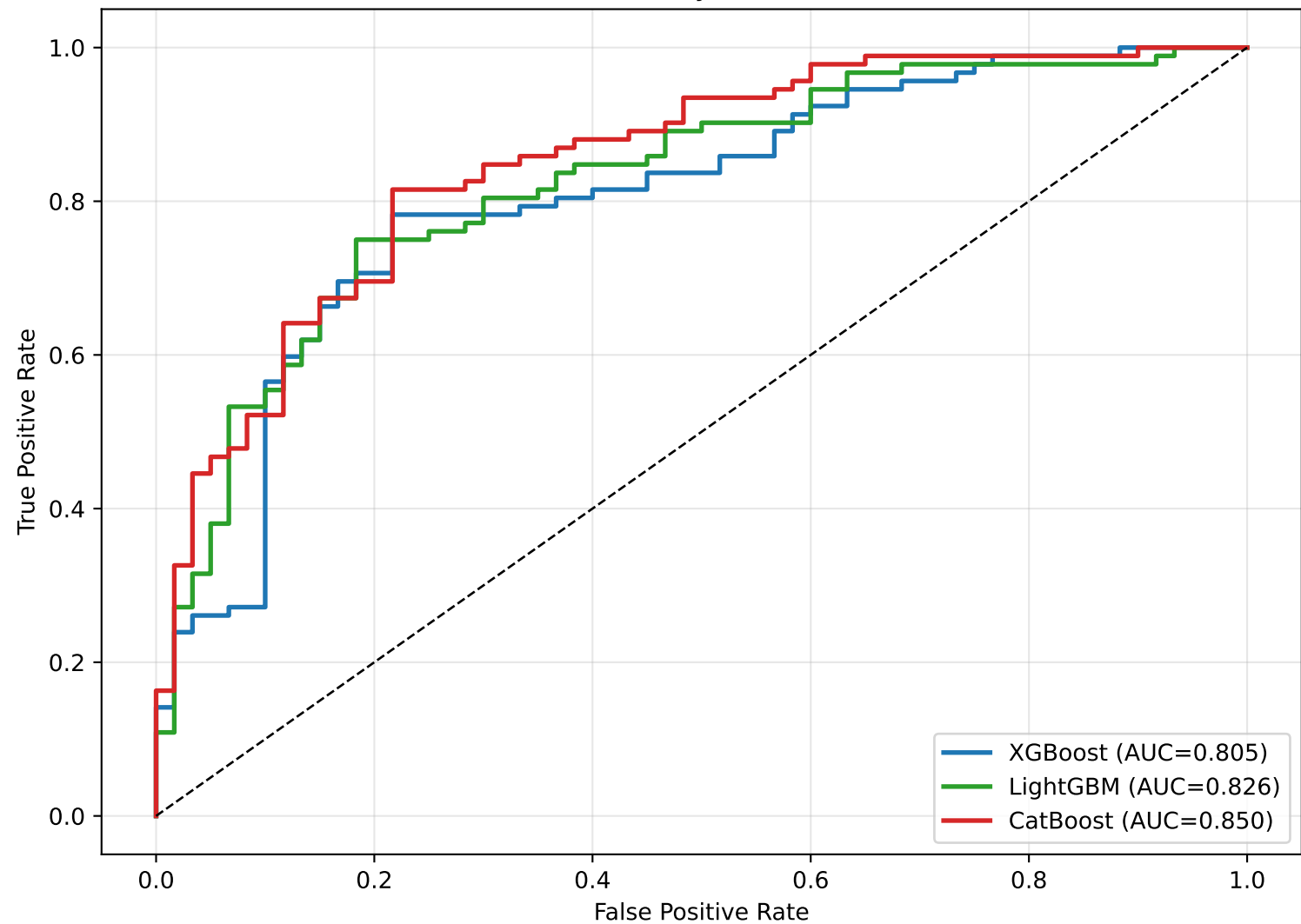
BACE PC-Only ROC Curves
