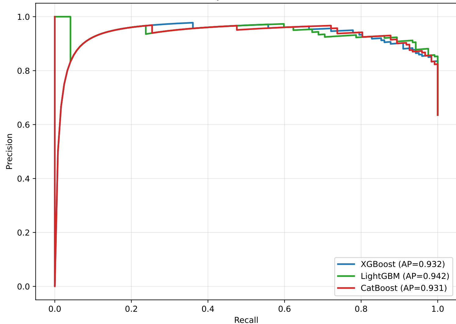
BBBP PC-Only Precision-Recall Curves
