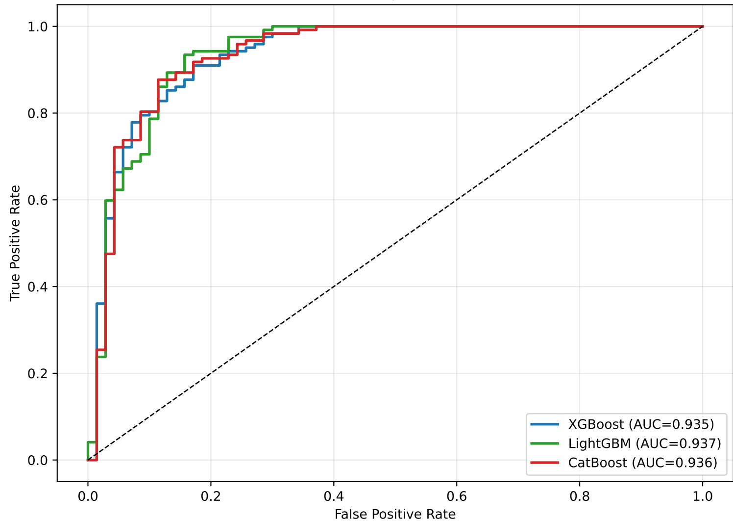
BBBP PC-Only ROC Curves
