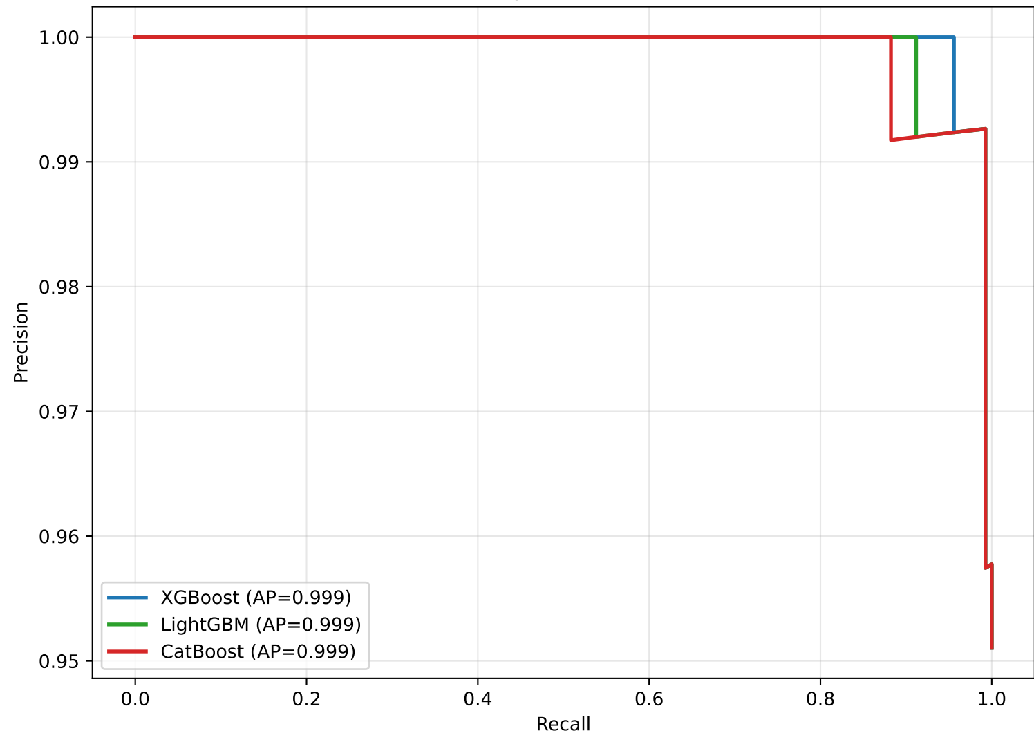
CLINTOX PC-Only Precision-Recall Curves
