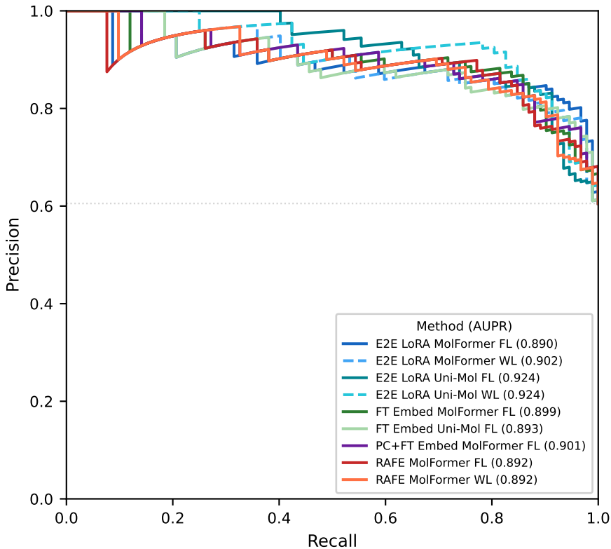
PR Curves — BACE
