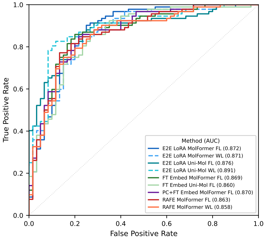
ROC Curves — BACE
