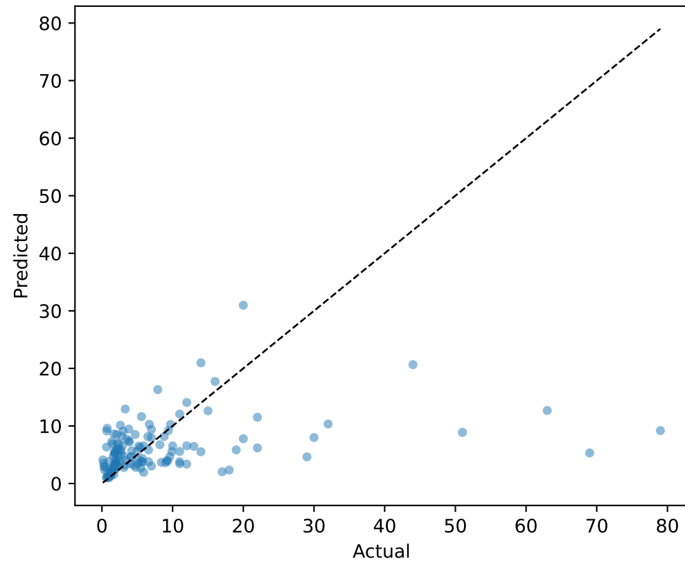
XGBoost (R2=0.110)
