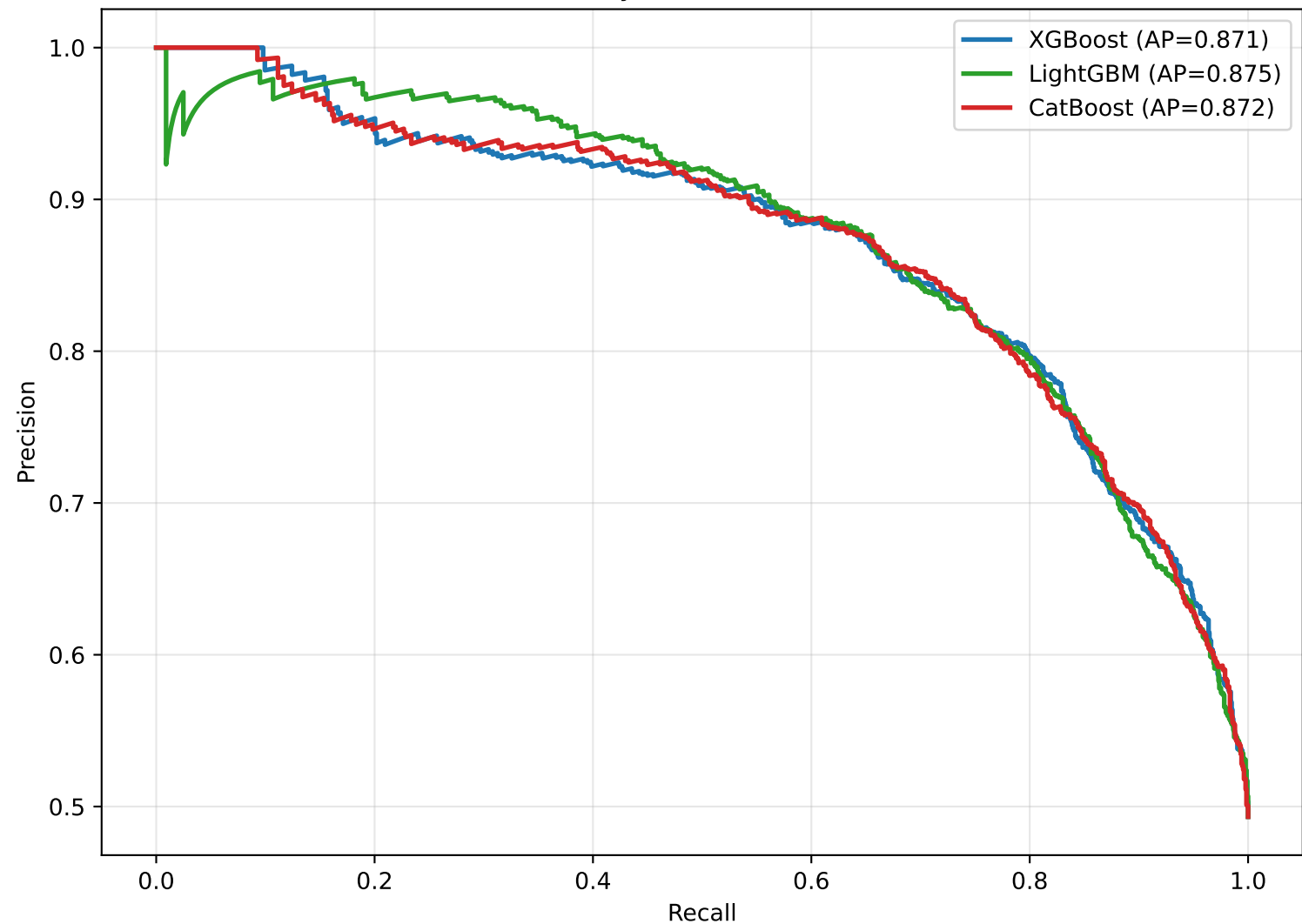
HERG PC-Only Precision-Recall Curves
