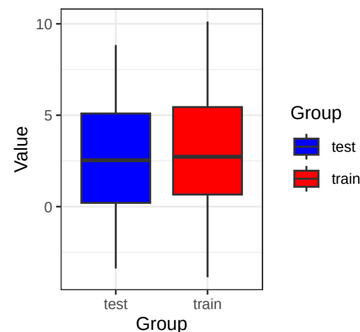
AHSP (Wilcoxon p= 0.746 )
