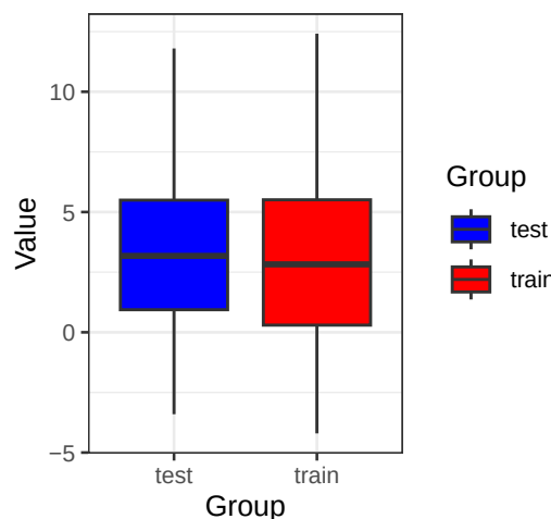
SCN9A.x (Wilcoxon p= 0.529 )
