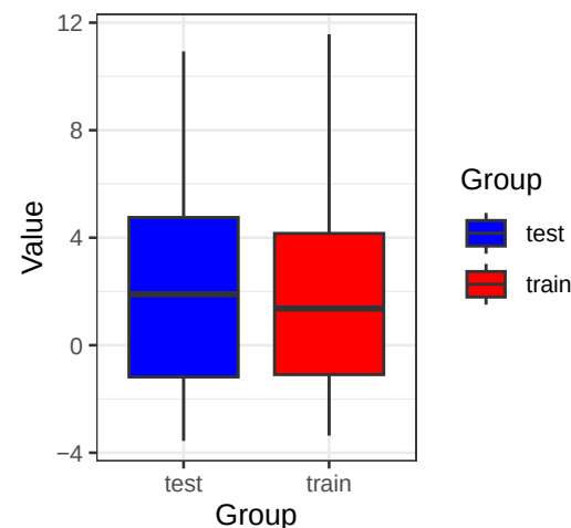
CDH2 (Wilcoxon p= 0.813 )
