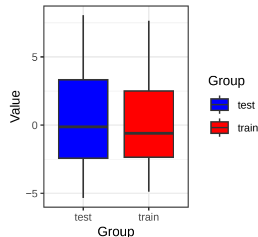
IRX5 (Wilcoxon p= 0.599 )
