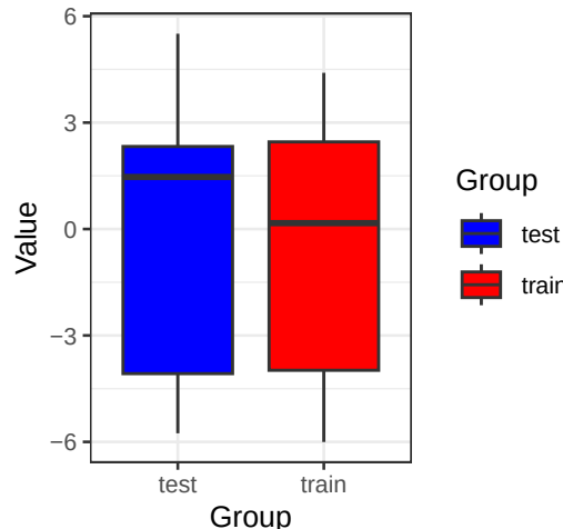
TTY14 (Wilcoxon p= 0.788 )
