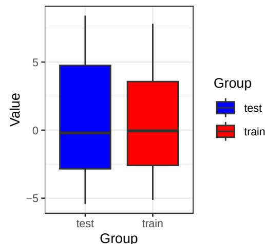
IRX3 (Wilcoxon p= 0.829 )
