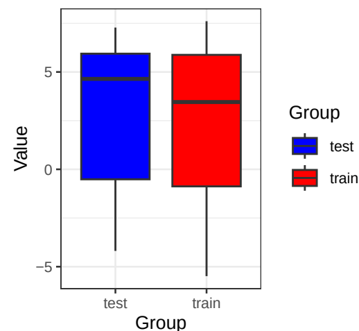
ARPP21 (Wilcoxon p= 0.312 )
