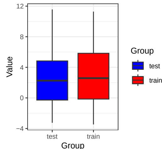
CD34 (Wilcoxon p= 0.343 )
