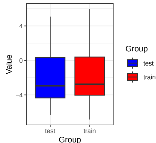
CDH4 (Wilcoxon p= 0.502 )
