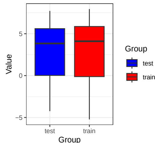
DPP10 (Wilcoxon p= 0.743 )
