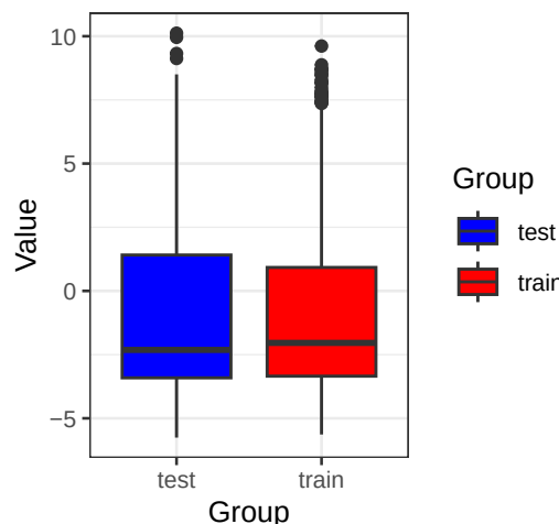
CSPG4 (Wilcoxon p= 0.0291 )
