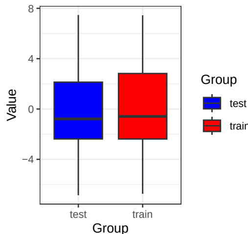
HOXB9 (Wilcoxon p= 0.649 )
