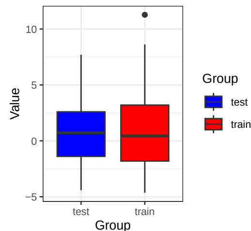
RXFP1 (Wilcoxon p= 0.72 )
