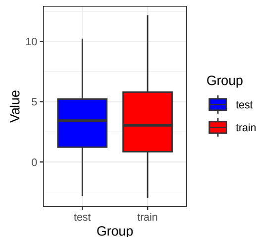
TRH (Wilcoxon p= 0.126 )
