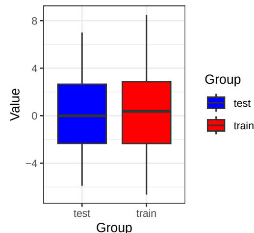
C20orf166-AS1 (Wilcoxon p= 0. )
