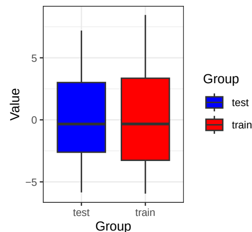
LINC00982 (Wilcoxon p= 0.281 )
