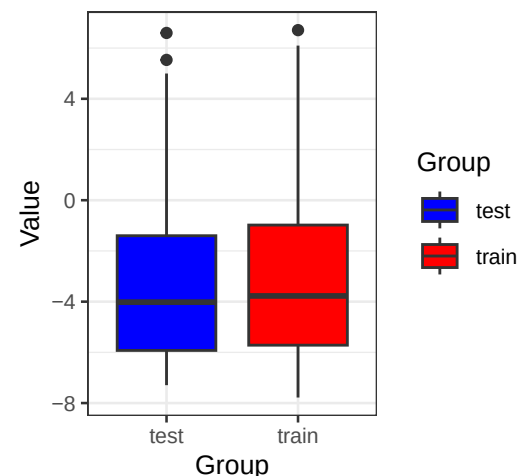
KCNE1L (Wilcoxon p= 0.607 )
