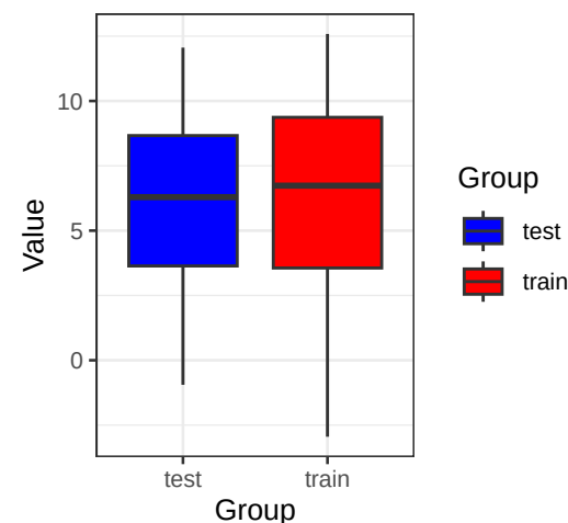
GYPA (Wilcoxon p= 0.798 )
