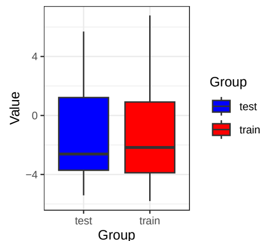
LAMB2 (Wilcoxon p= 0.793 )
