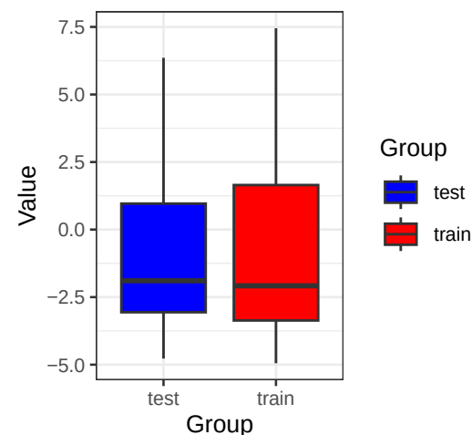
GTSF1 (Wilcoxon p= 0.131 )
