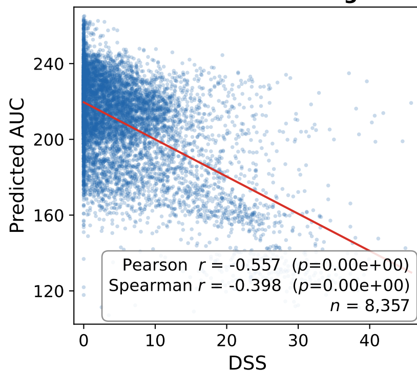
SMILES Embedding
