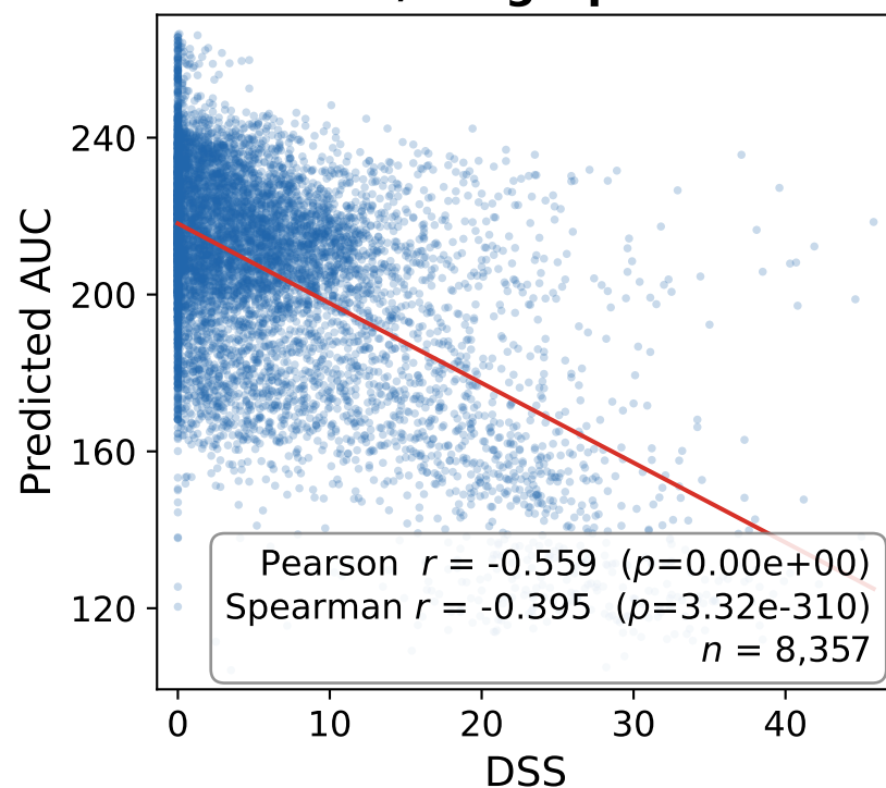
PC / Fingerprints
