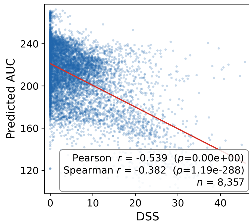
MolFormer
