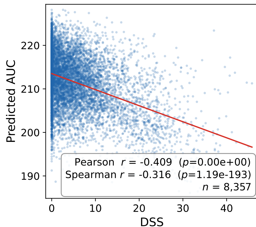
ChemBERTa
