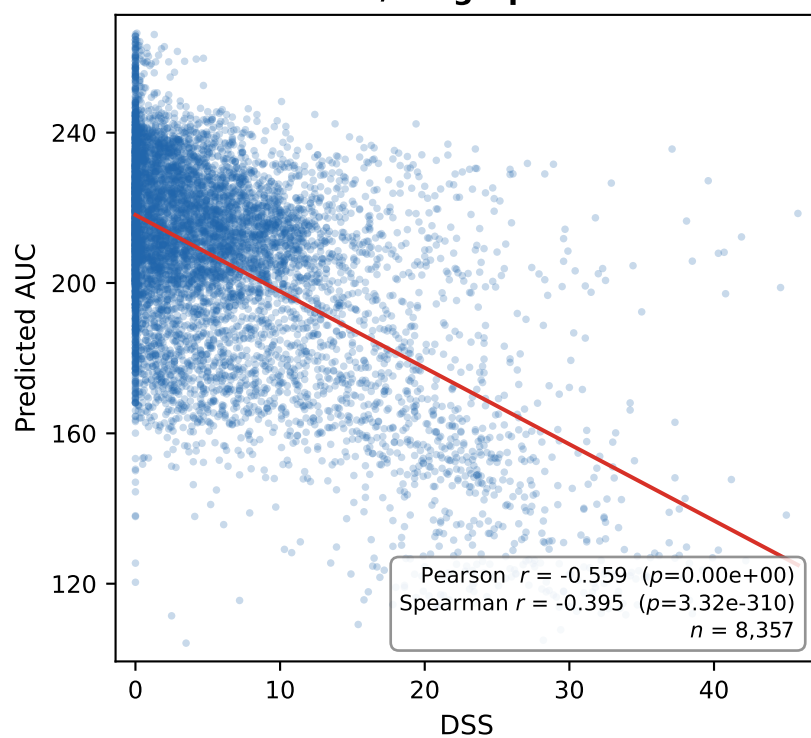
PC / Fingerprints
