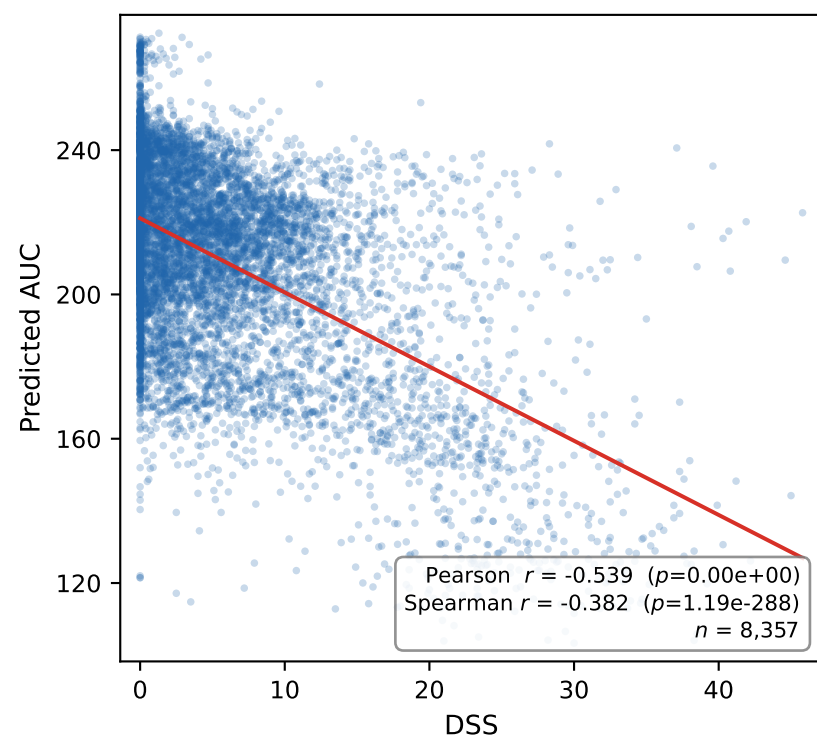
MolFormer
