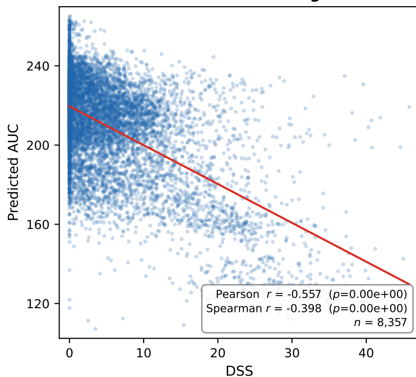
SMILES Embedding
