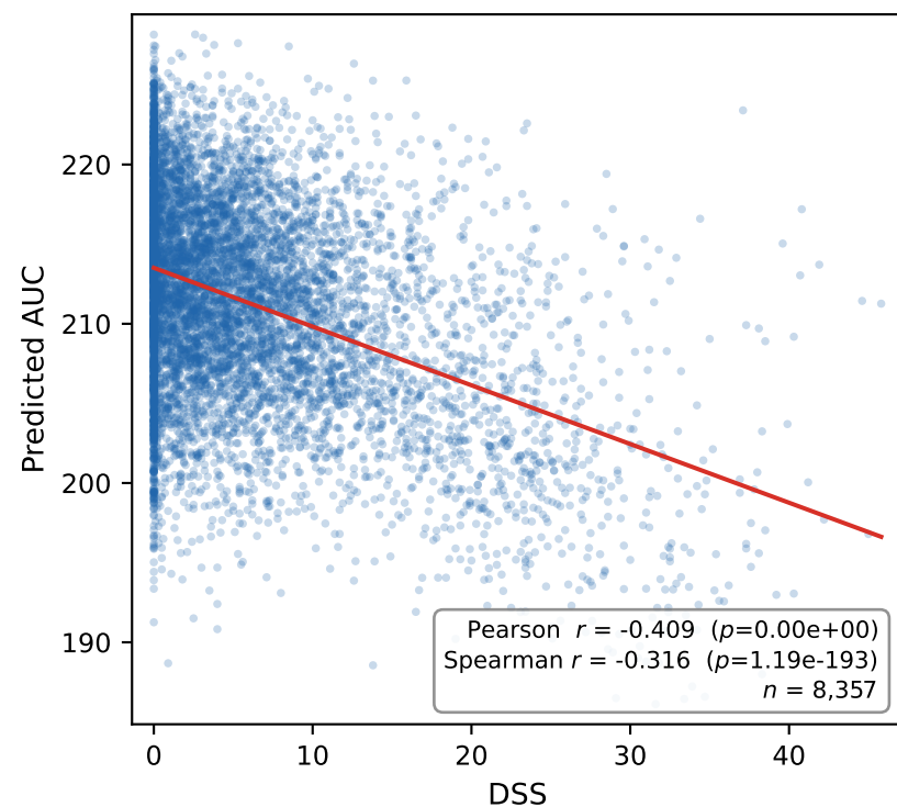
ChemBERTa
