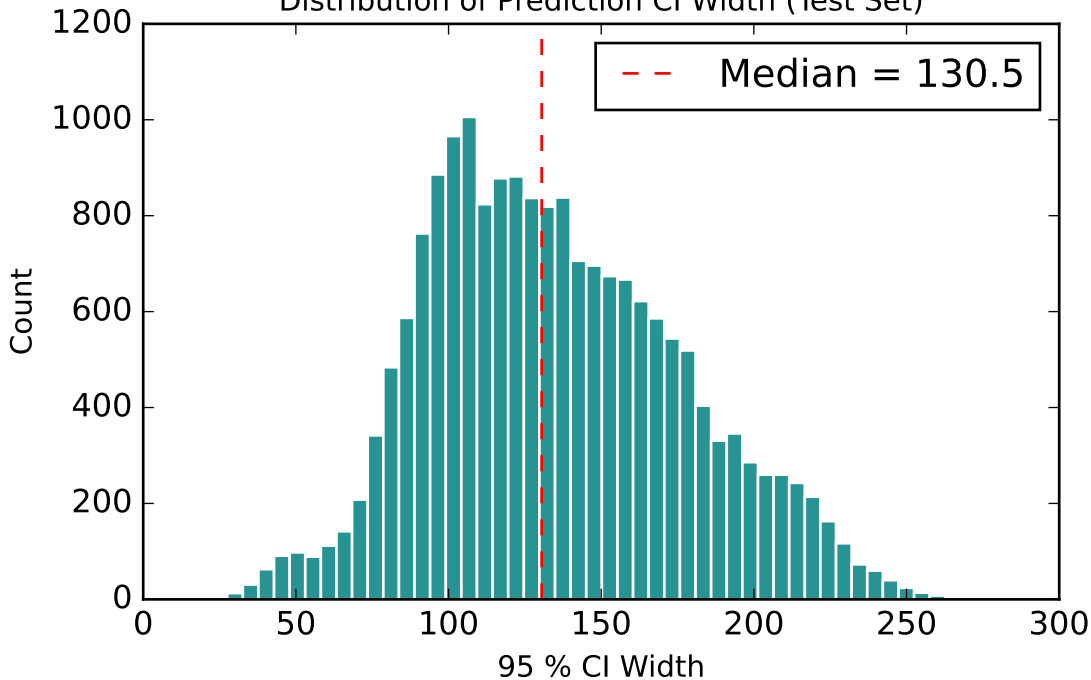
Distribution of Prediction CI Width (Test Set)
