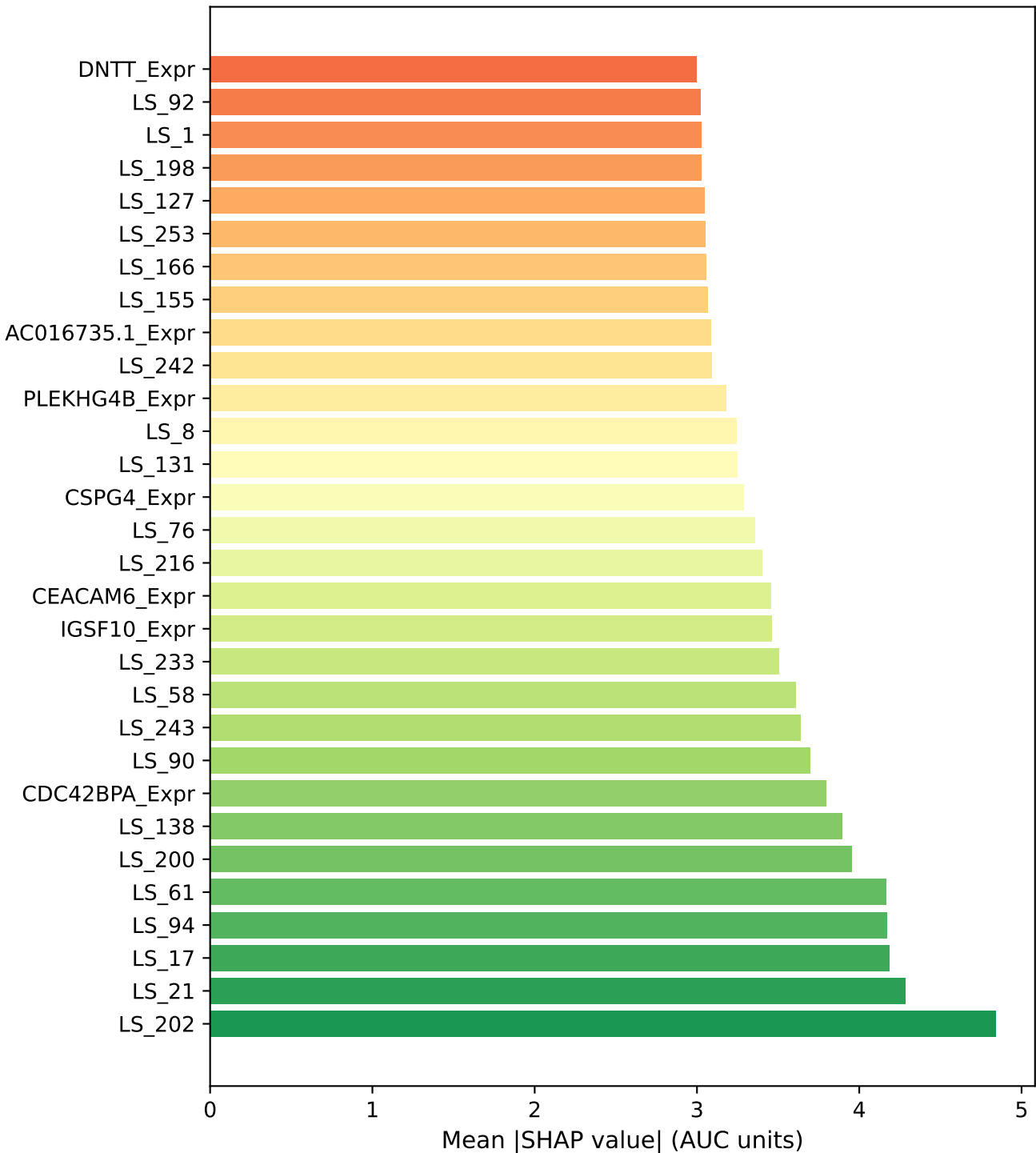
Top 30 SHAP Feature Importance - Test
