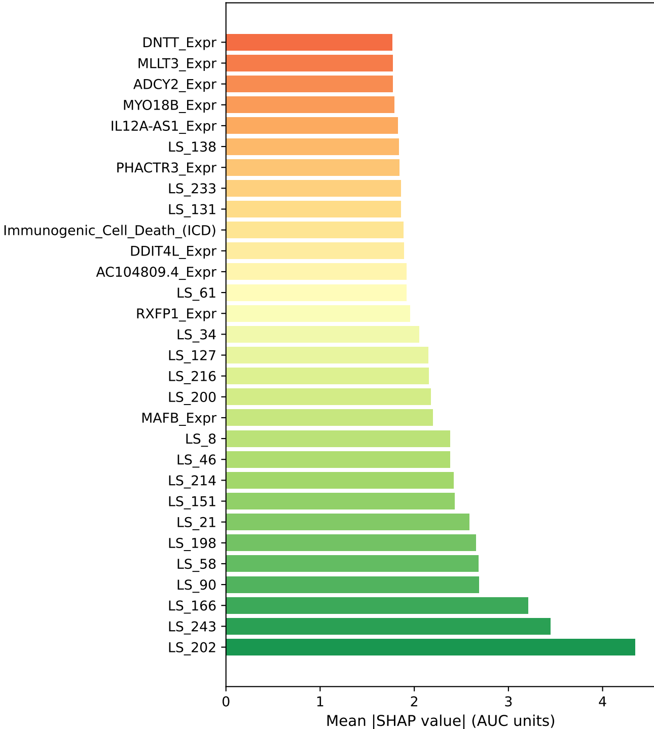
Top 30 SHAP Feature Importance - Train
