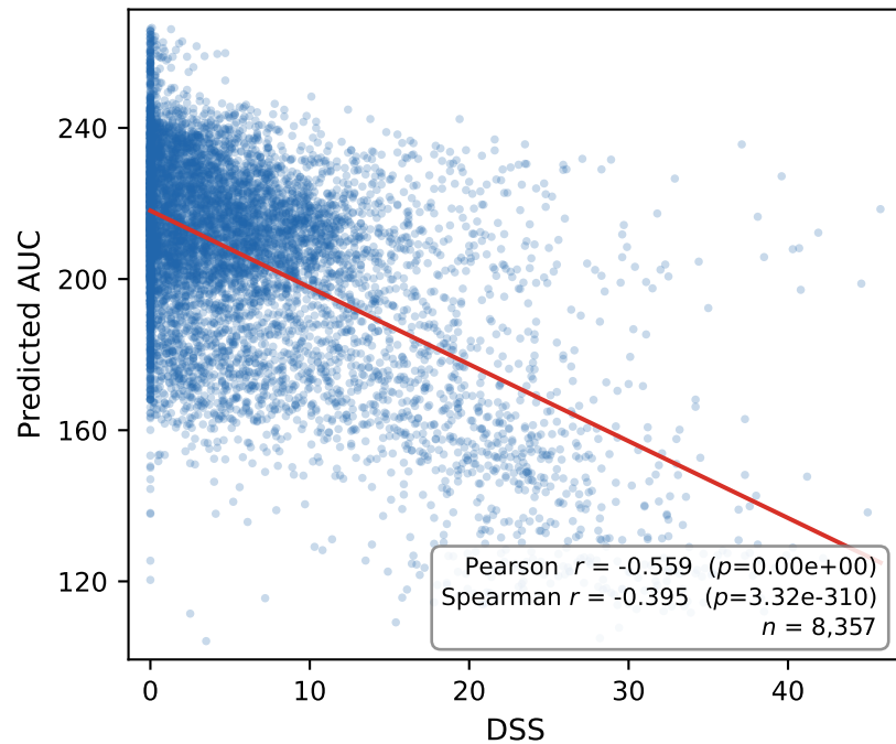
PC / Fingerprints
