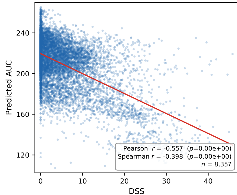
SMILES Embedding
