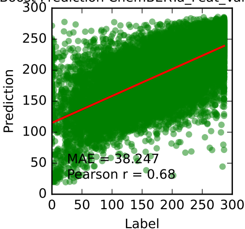
CatBoost Prediction ChemBERTa_Feat_Var_inhibitor
