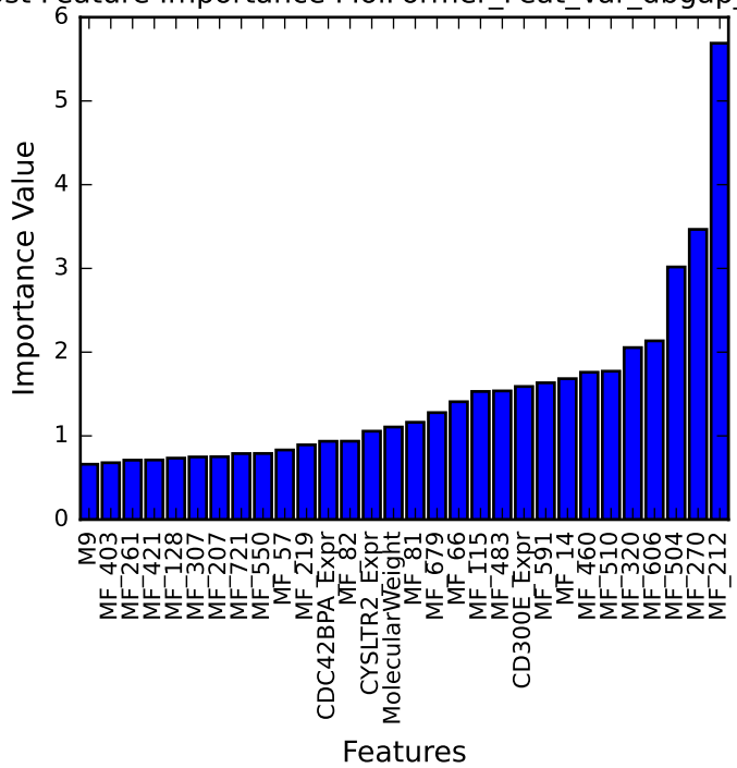
Top CatBoost Feature Importance MolFormer_Feat_Var_dbgap_rnaseq_sample
