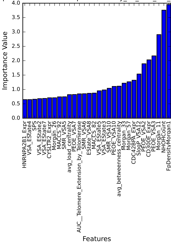
Top CatBoost Feature Importance Only_PC_Feat_Var_inhibitor
