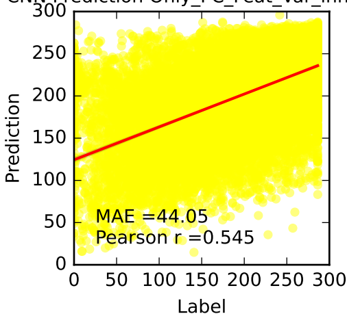
CNN Prediction Only_PC_Feat_Var_inhibitor
