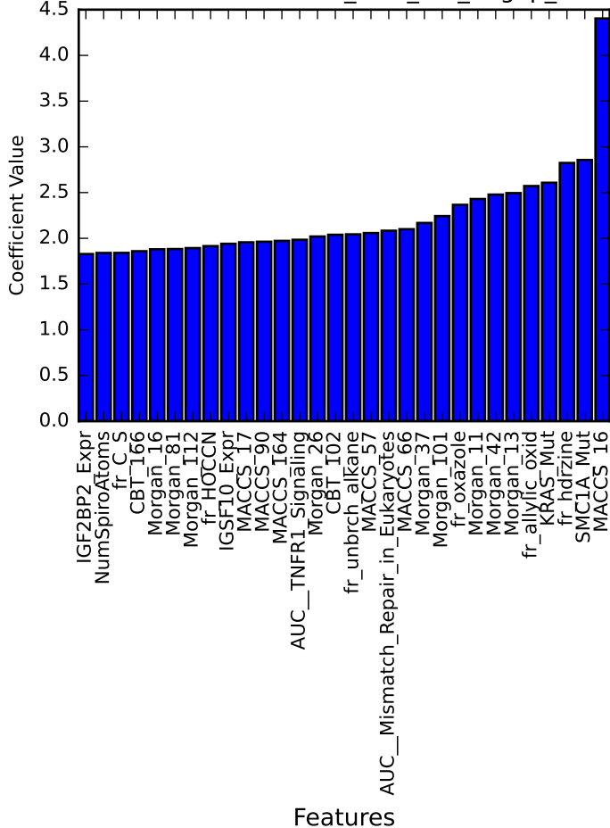
Top GLR Coefficients ChemBERTa_Feat_Var_dbgap_rnaseq_sample
