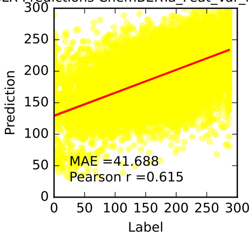
GLR Predictions ChemBERTa_Feat_Var_inhibitor
