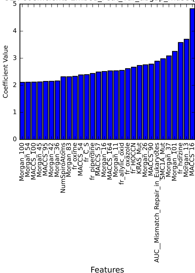
Top GLR Coefficients Embed_Feat_Var_dbgap_rnaseq_sample
