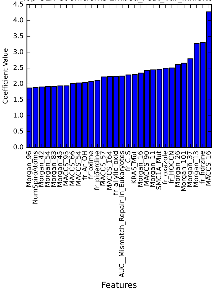
Top GLR Coefficients Embed_Feat_Var_inhibitor
