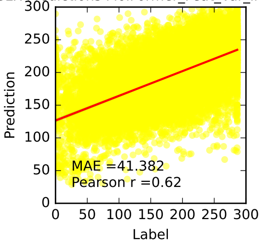
GLR Predictions MolFormer_Feat_Var_inhibitor
