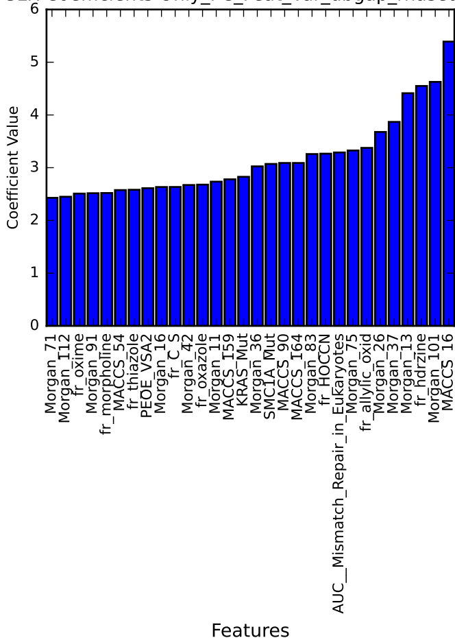
Top GLR Coefficients Only_PC_Feat_Var_dbgap_rnaseq_sample
