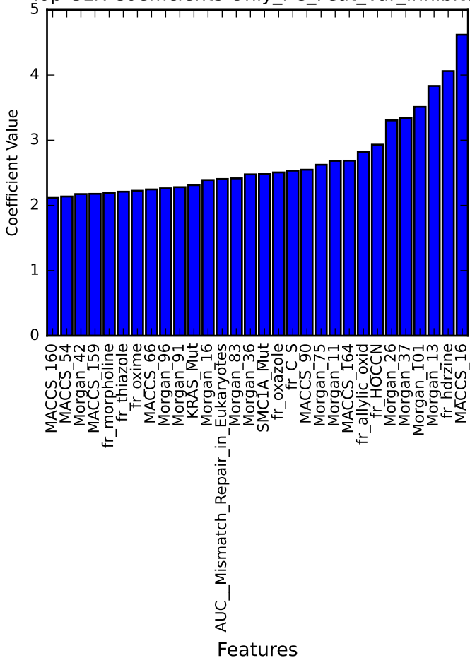
Top GLR Coefficients Only_PC_Feat_Var_inhibitor
