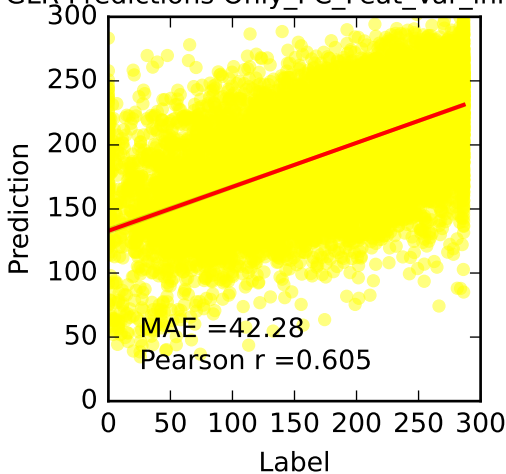
GLR Predictions Only_PC_Feat_Var_inhibitor
