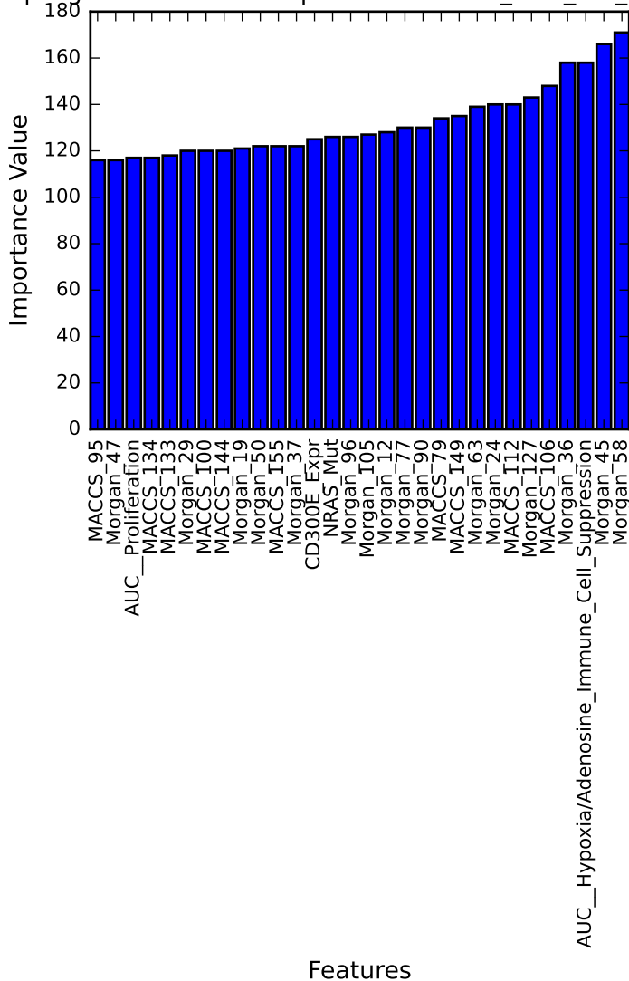
Top LightGBM Feature Importance Embed_Feat_Var_random
