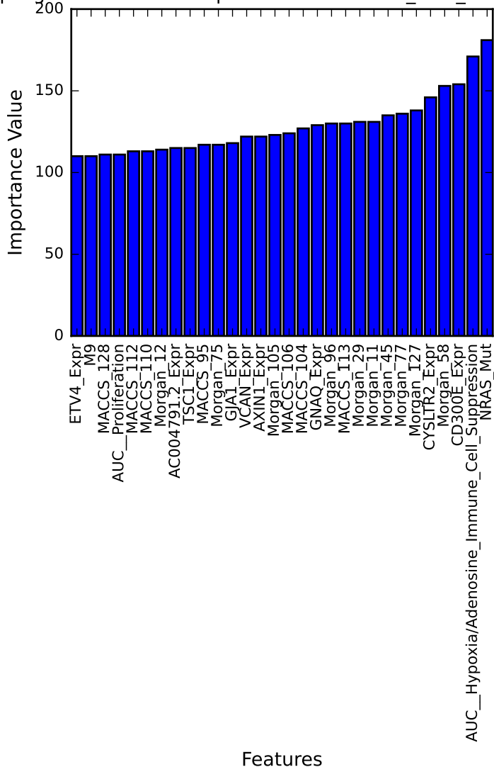
Top LightGBM Feature Importance MolFormer_Feat_Var_inhibitor
